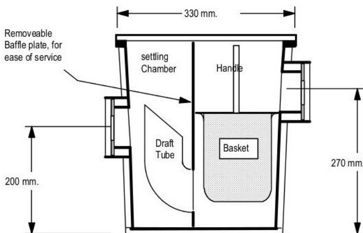
<< Section through a 24L trap
